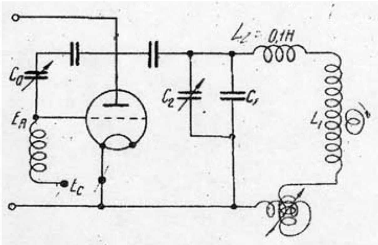
Figure 9: Circuit for parametric excitation in a system with regeneration
